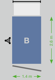
Landing level safety gate
